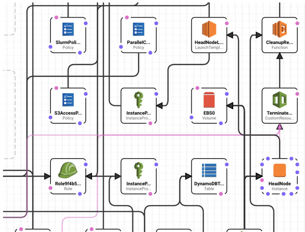
Fig. 9.1: AWS ParallelCluster sets up a CloudFormation stack to deploy all the resources you need to run your cluster on AWS automatically, and easily.
